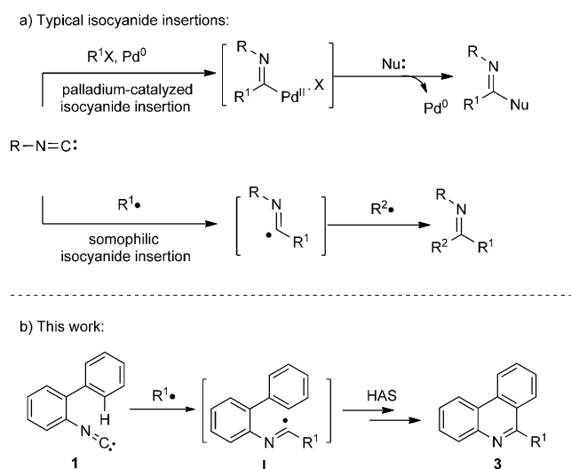
Scheme 1. Typical isocyanide insertions and our design.
